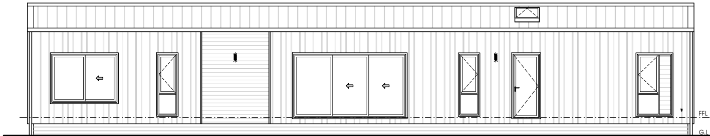
ELEVATE BARN 154 SHOWHOME - ELEVATIONS
